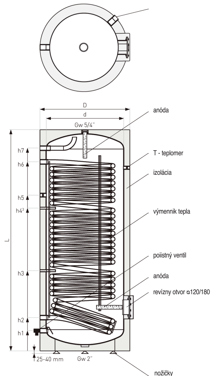
QUADROFLEX QFDS 1 200 P
