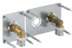
MOUNTING PLATE ASSEMBLED WITH 2 WALLPLATE ELBOWS 90° DISTANCE 76 mm
